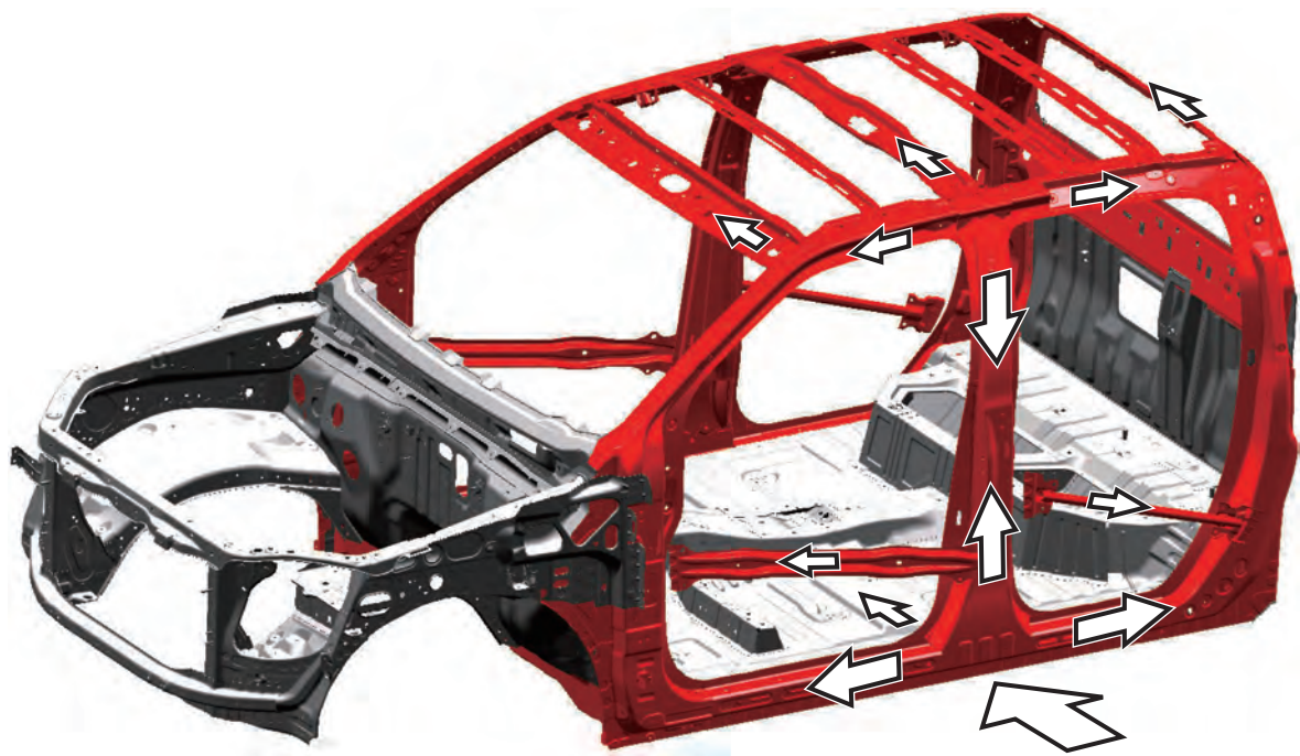
Crew Cab
