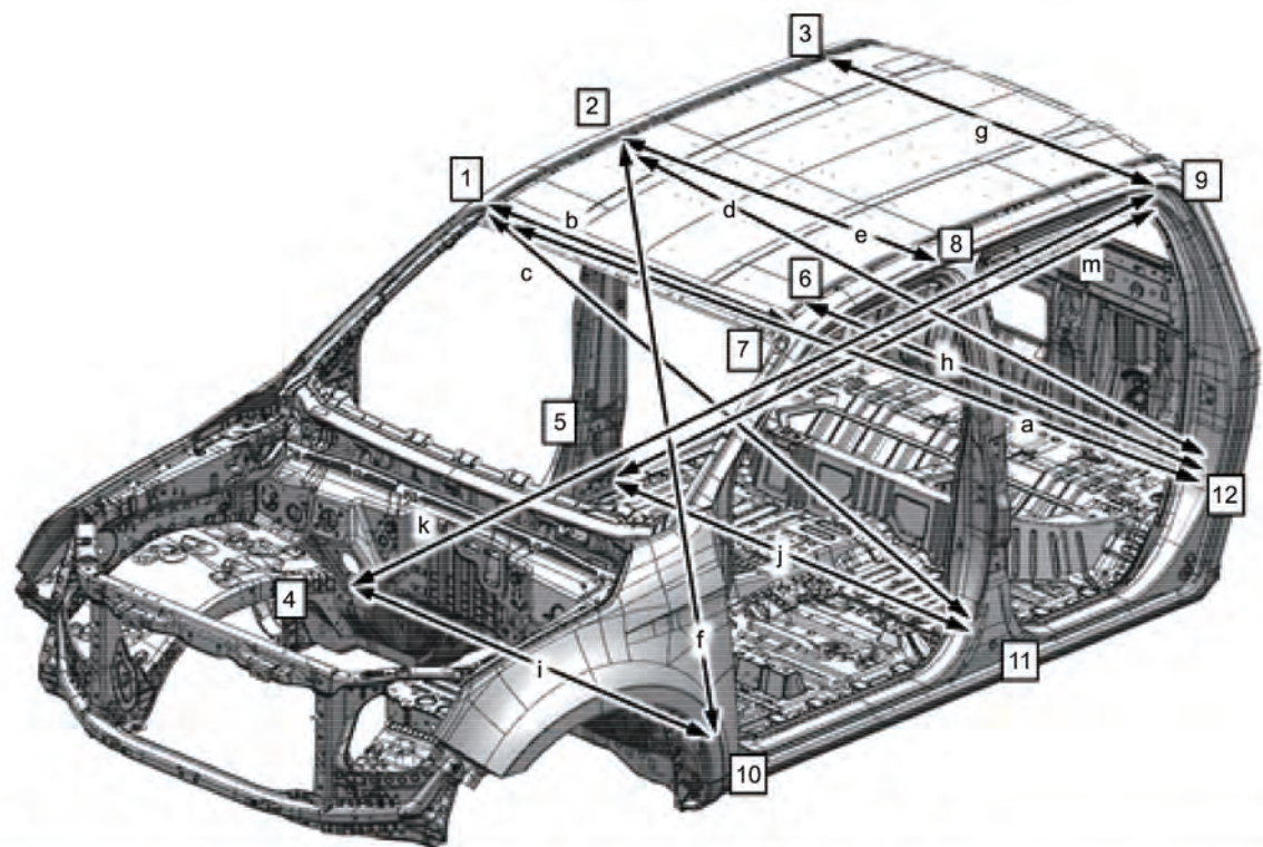
Crew cab body dimensions
