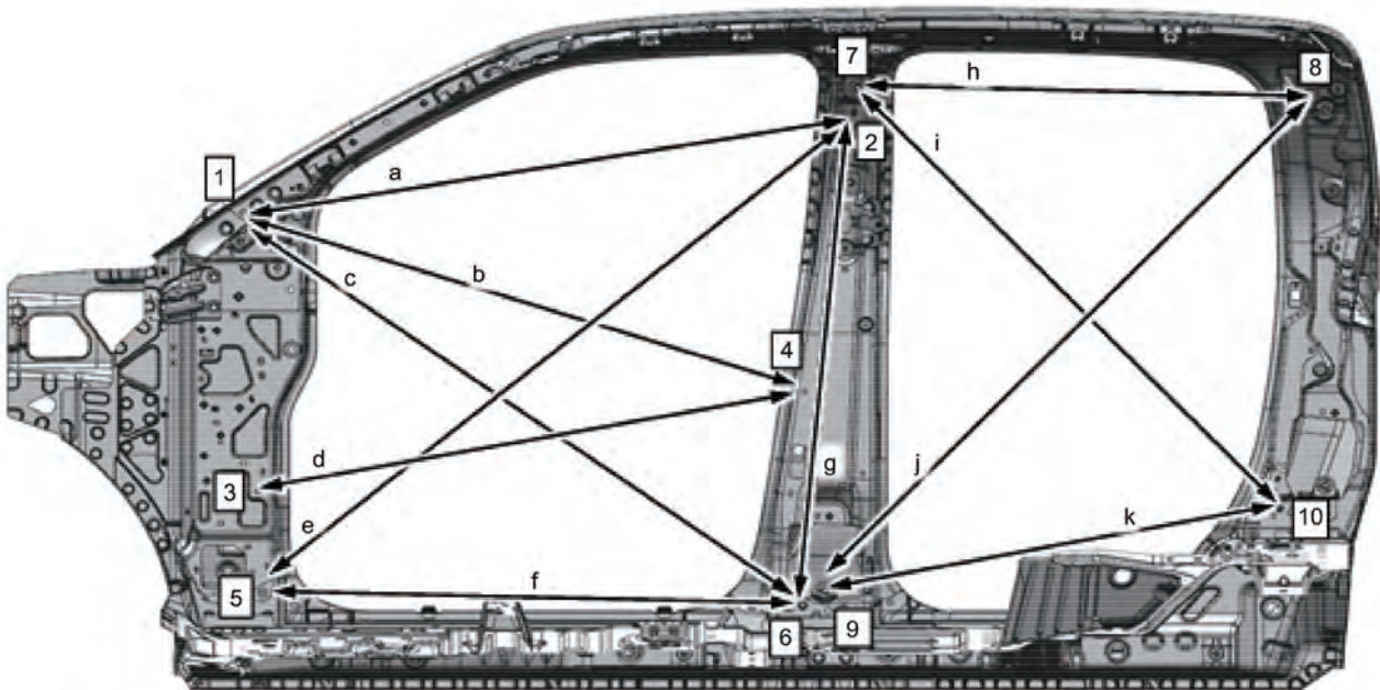
Crew cab body dimension
