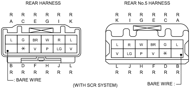
C-88 REAR No.5 HARNESS-SHORT CORD
