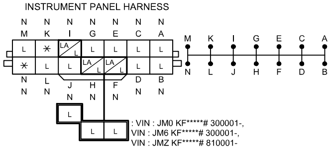
C-60 JOINT CONNECTOR
