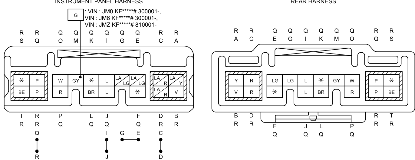
C-16 INSTRUMENT PANEL HARNESS-REAR HARNESS
