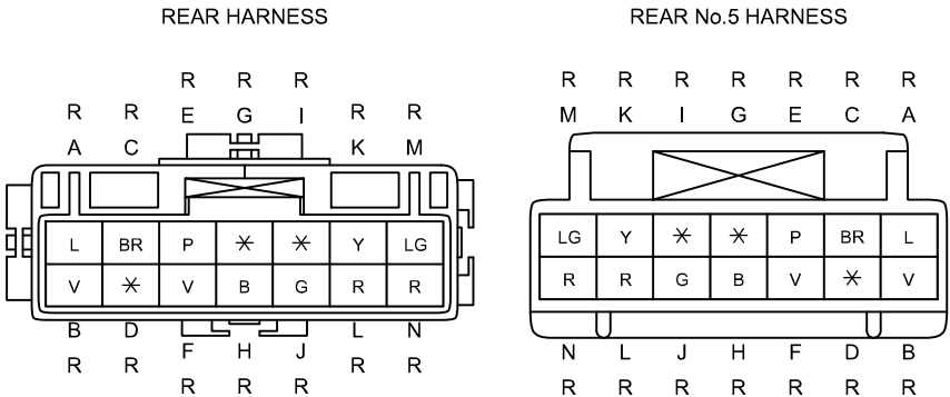
C-26 REAR HARNESS-REAR No.5 HARNESS
