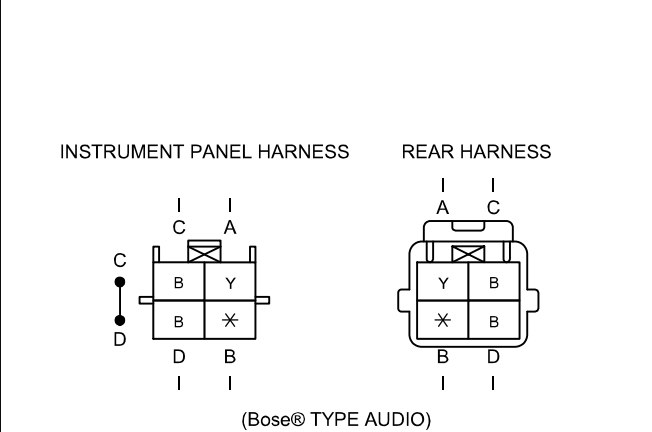
C-18 INSTRUMENT PANEL HARNESS-REAR HARNESS
