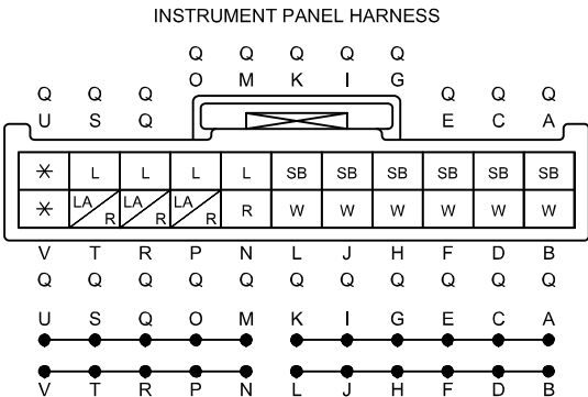
C-62 JOINT CONNECTOR
