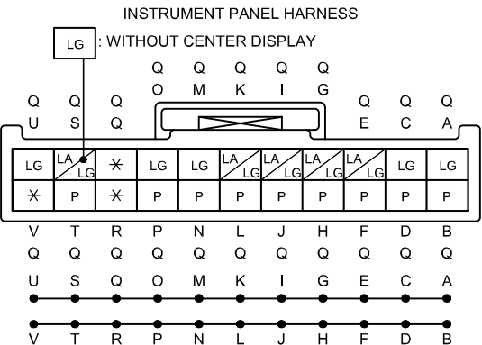
C-64 JOINT CONNECTOR
