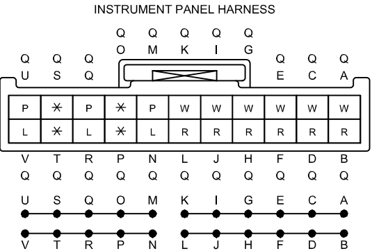
C-64 JOINT CONNECTOR
