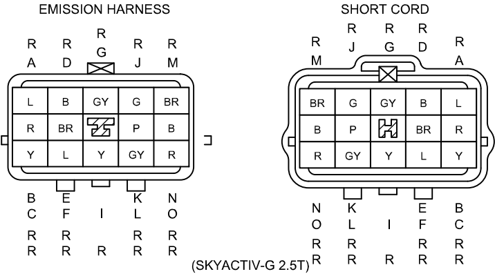
C-90 EMISSION HARNESS-SHORT CORD
