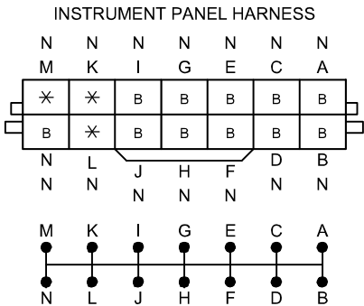
C-65 JOINT CONNECTOR
