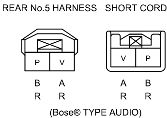
C-80 REAR No.5 HARNESS-SHORT CORD
