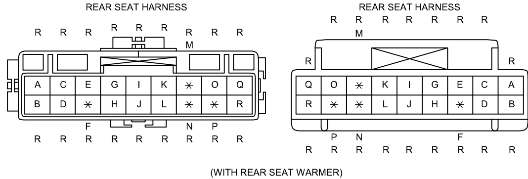
C-78 REAR SEAT HARNESS-REAR SEAT HARNESS
