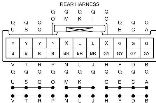
C-66 JOINT CONNECTOR
