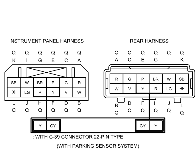
C-15 INSTRUMENT PANEL HARNESS-REAR HARNESS
