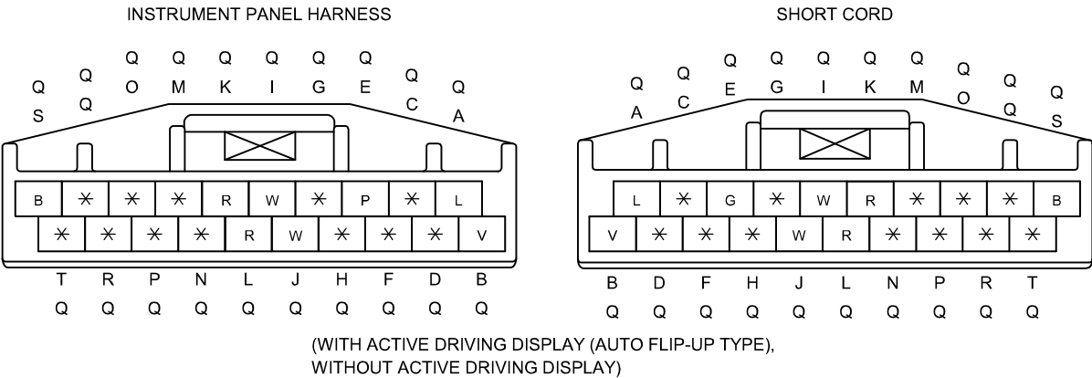
C-82 INSTRUMENT PANEL HARNESS-SHORT CORD
