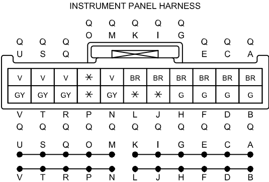
C-61 JOINT CONNECTOR
