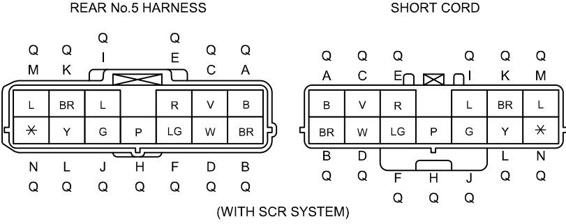
C-87 JOINT CONNECTOR
