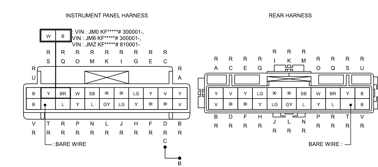
C-17 INSTRUMENT PANEL HARNESS-REAR HARNESS
