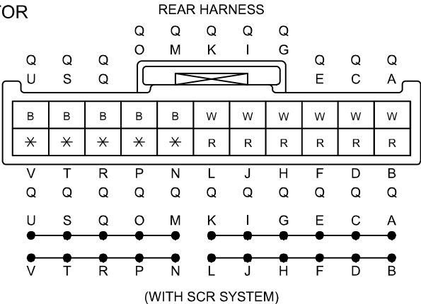
C-90 EMISSION HARNESS-SHORT CORD
