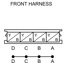
C-33 JOINT CONNECTOR
