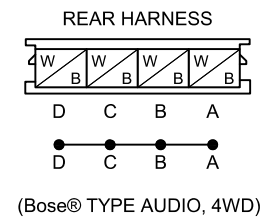
C-53 INSTRUMENT PANEL HARNESS-SHORT CORD
