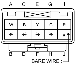
INSTRUMENT PANEL HARNESS
