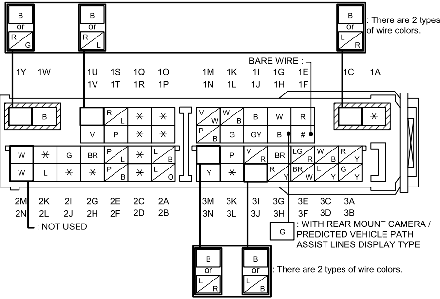
REAR NO.5 HARNESS
