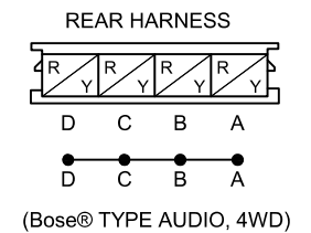
C-54 JOINT CONNECTOR
