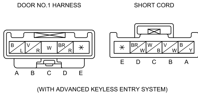
C-30 DOOR NO.1 HARNESS-SHORT CORD
