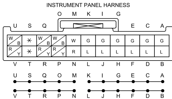
C-37 JOINT CONNECTOR
