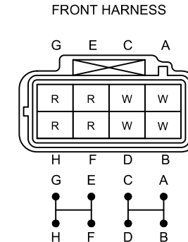
C-32 JOINT CONNECTOR
