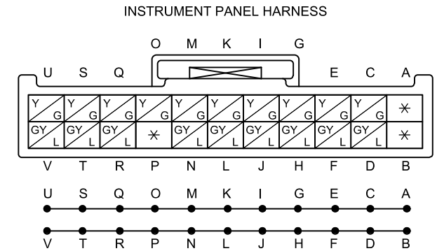
C-39 INSTRUMENT PANEL HARNESS- REAR HARNESS
