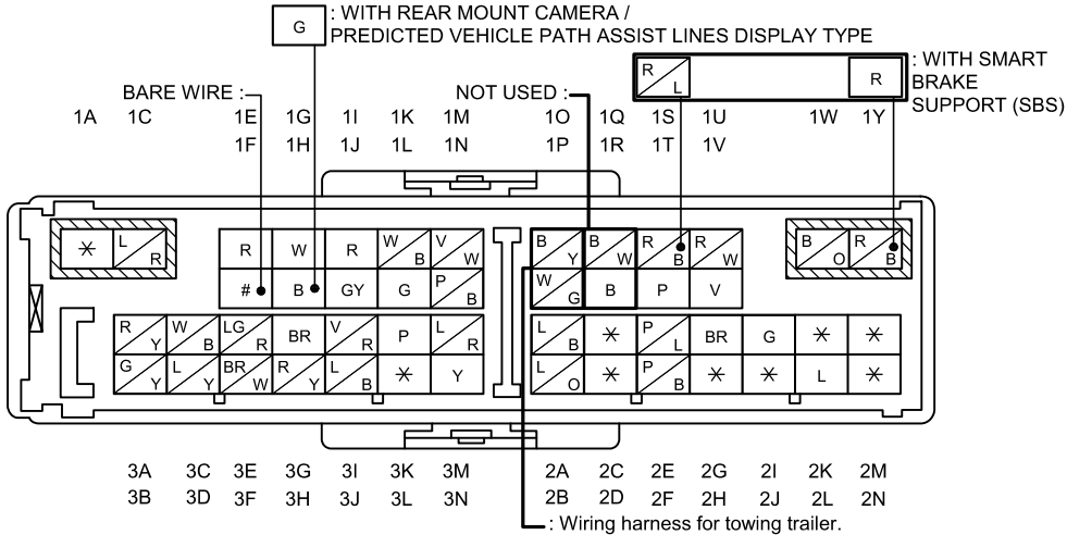
REAR HARNESS
