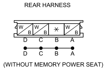
C-55 JOINT CONNECTOR
