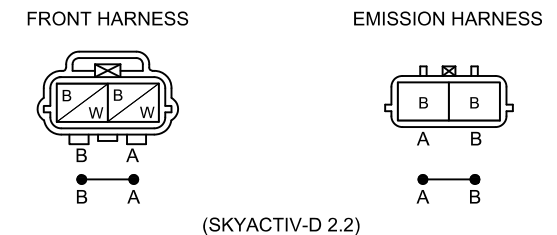
C-58 FRONT HARNESS-EMISSION HARNESS
