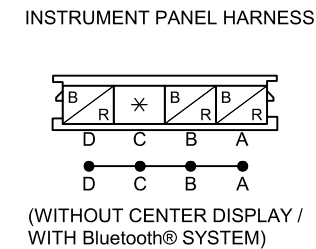
C-49 JOINT CONNECTOR
