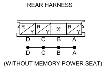
C-56 REAR HARNESS-SHORT CORD
