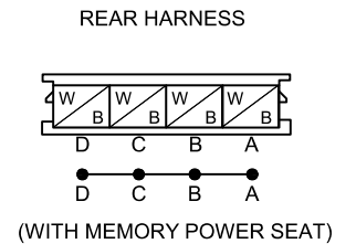
C-54 JOINT CONNECTOR
