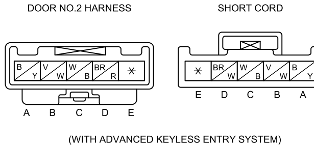
C-35 JOINT CONNECTOR
