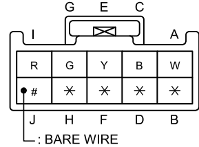
INTERIOR LIGHT NO.2 HARNESS
