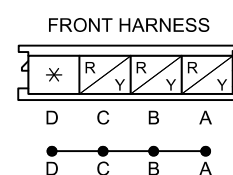
C-57 JOINT CONNECTOR
