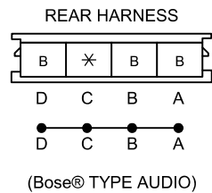
C-51 JOINT CONNECTOR
