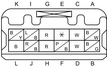
INTERIOR LIGHT NO.2 HARNESS
