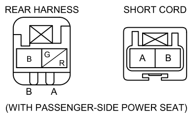
C-56 REAR HARNESS-SHORT CORD
