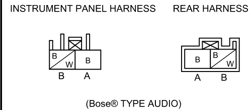
C-39 INSTRUMENT PANEL HARNESS- REAR HARNESS
