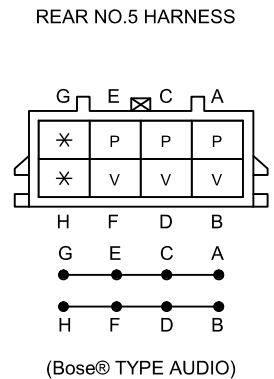
C-40 JOINT CONNECTOR
