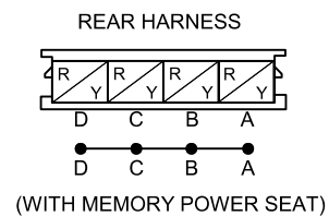
C-55 JOINT CONNECTOR
