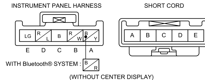
C-57 JOINT CONNECTOR
