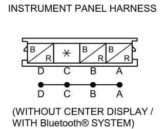
C-50 JOINT CONNECTOR
