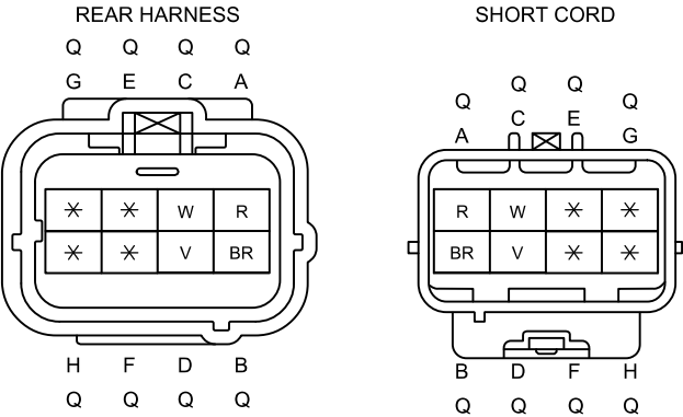
C-34 REAR HARNESS-SHORT CORD
