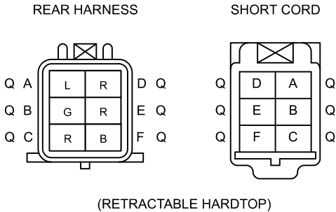
C-49 REAR HARNESS-SHORT CORD
