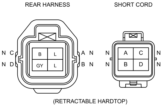
C-50 REAR HARNESS-SHORT CORD
