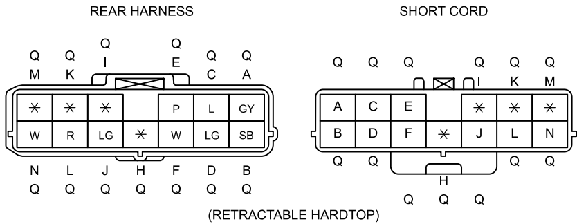
C-47 REAR HARNESS-SHORT CORD
