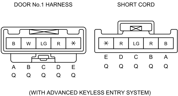
C-39 JOINT CONNECTOR
