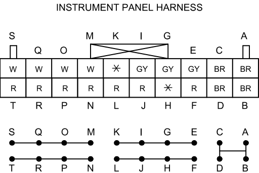
C-40 JOINT CONNECTOR
