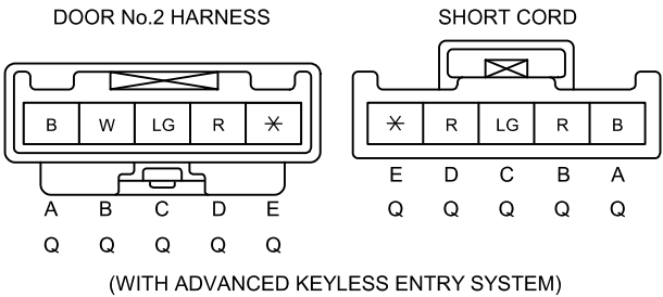
C-37 DOOR No.2 HARNESS-SHORT CORD
