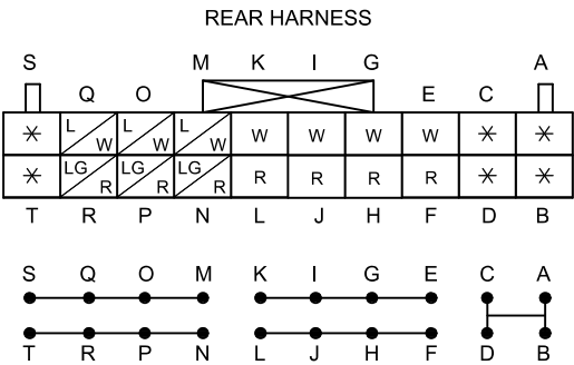
C-42 JOINT CONNECTOR
