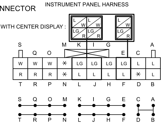
C-42 JOINT CONNECTOR
