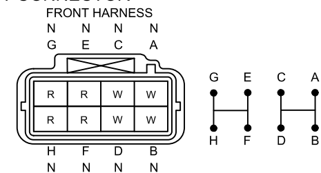
C-33 JOINT CONNECTOR
