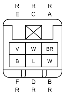
DOOR No.1 HARNESS
