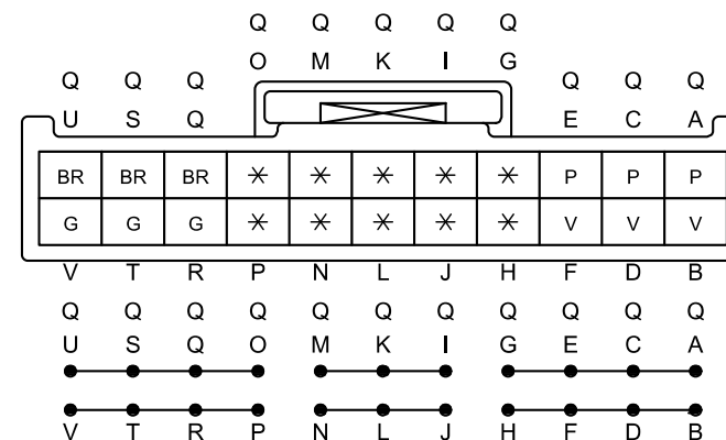
INSTRUMENT PANEL HARNESS
