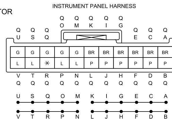
C-32 JOINT CONNECTOR
