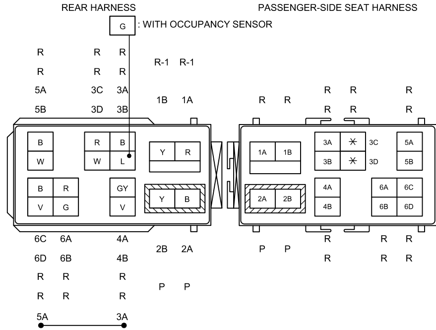
C-20 REAR HARNESS-PASSENGER-SIDE SEAT HARNESS
