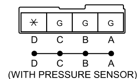
C-51 JOINT CONNECTOR
