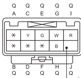
INTERIOR LIGHT No.2 HARNESS
