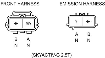
C-60 JOINT CONNECTOR
