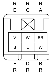
DOOR No.2 HARNESS
