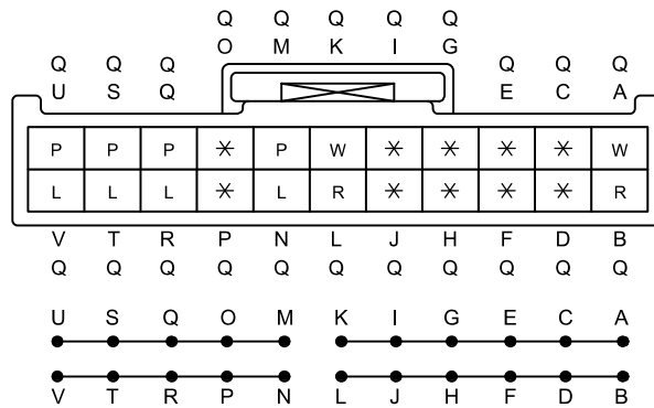
C-37 JOINT CONNECTOR
