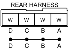
C-60 JOINT CONNECTOR
