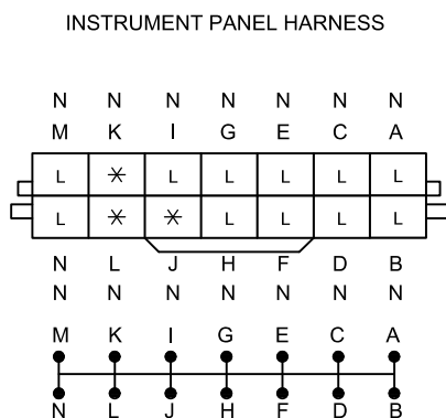
C-29 JOINT CONNECTOR
