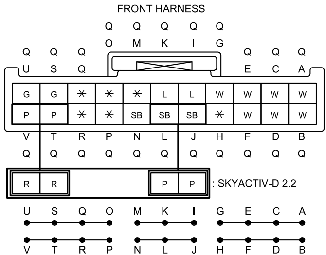
C-62 JOINT CONNECTOR
