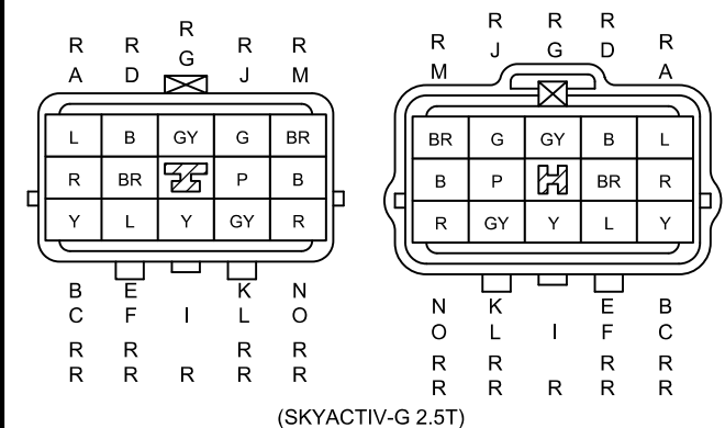
C-43 JOINT CONNECTOR
