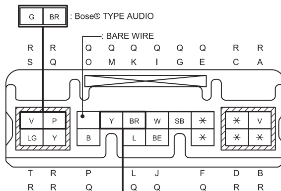
INSTRUMENT PANEL HARNESS
