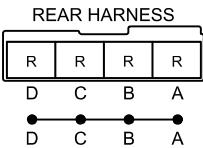
C-59 JOINT CONNECTOR
