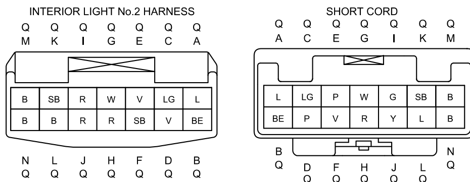
C-29 JOINT CONNECTOR
