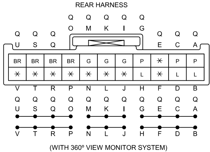
C-63 JOINT CONNECTOR
