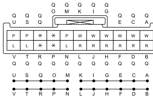
C-38 JOINT CONNECTOR
