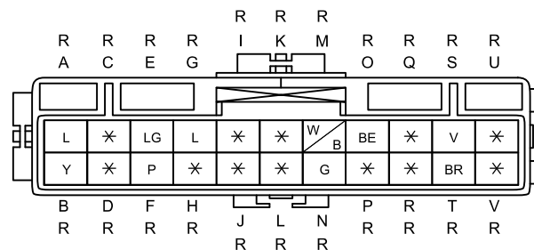
C-52 JOINT CONNECTOR
