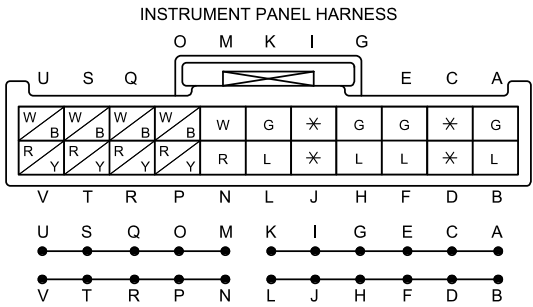
C-34 JOINT CONNECTOR
