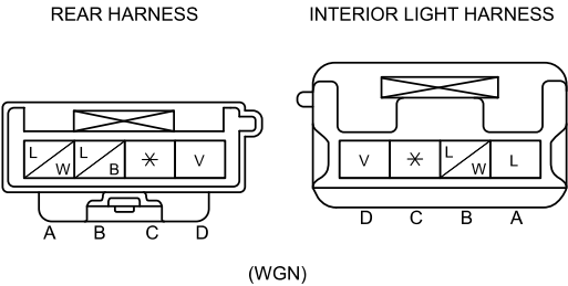
C-29 JOINT CONNECTOR
