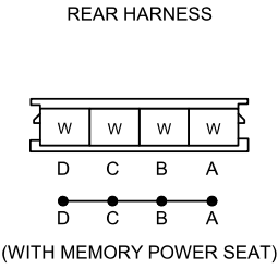
C-51 JOINT CONNECTOR
