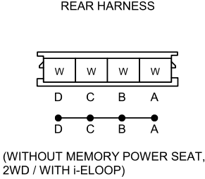
C-49 JOINT CONNECTOR
