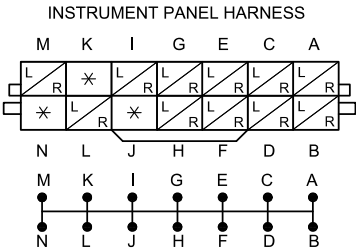
C-32 JOINT CONNECTOR
