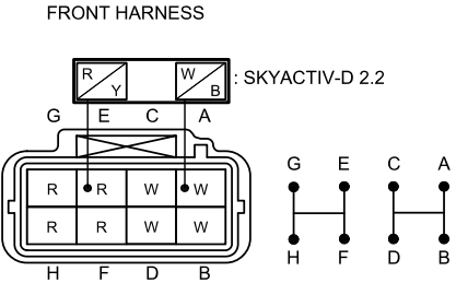
C-32 JOINT CONNECTOR
