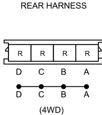
C-59 JOINT CONNECTOR
