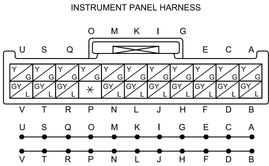
C-36 JOINT CONNECTOR
