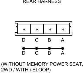
C-50 JOINT CONNECTOR
