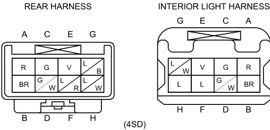
C-28 REAR NO.4 HARNESS-SHORT CORD
