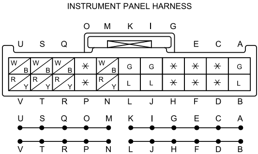
C-35 JOINT CONNECTOR
