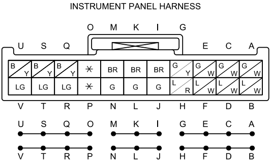
C-41 JOINT CONNECTOR
