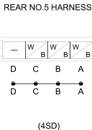
C-48 JOINT CONNECTOR
