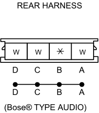
C-58 JOINT CONNECTOR
