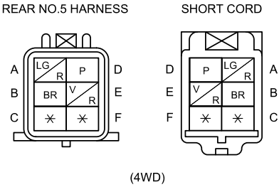
C-47 REAR NO.5 HARNESS-SHORT CORD
