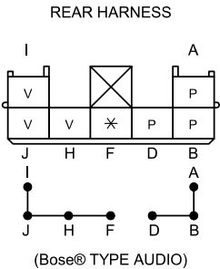
C-30 DOOR NO.1 HARNESS-SHORT CORD
