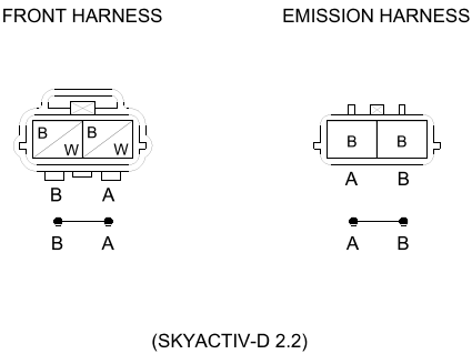
C-50 JOINT CONNECTOR
