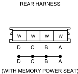
C-51 JOINT CONNECTOR
