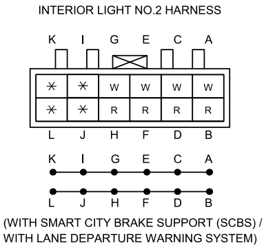
C-42 JOINT CONNECTOR
