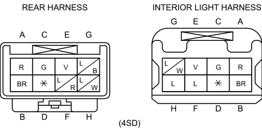
C-27 INTERIOR LIGHT NO.2 HARNESS-SHORT CORD
