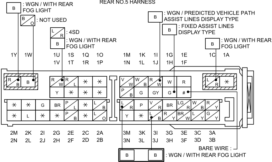
REAR NO.5 HARNESS
