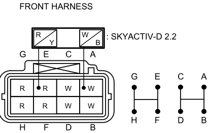
C-32 JOINT CONNECTOR
