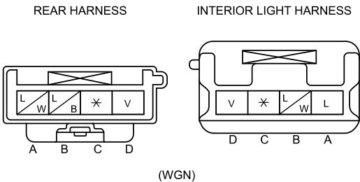
C-28 REAR NO.4 HARNESS-SHORT CORD
