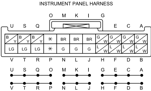
C-38 JOINT CONNECTOR
