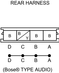
C-41 JOINT CONNECTOR
