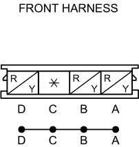
C-40 JOINT CONNECTOR
