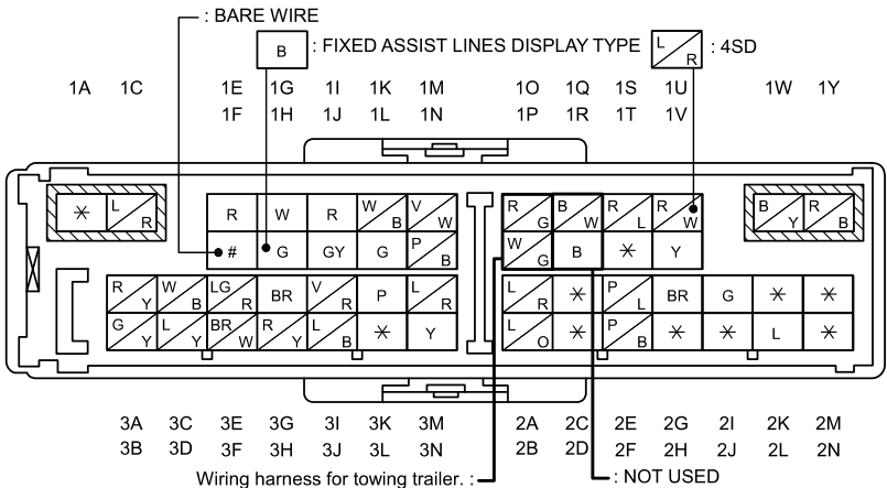
REAR HARNESS
