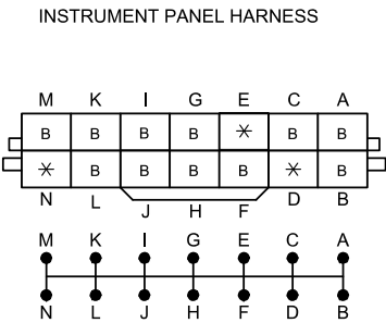
C-40 JOINT CONNECTOR
